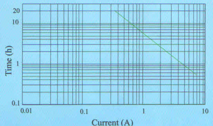
DISCHARGE CURRENT VS TIME 25! aC (77!a)
