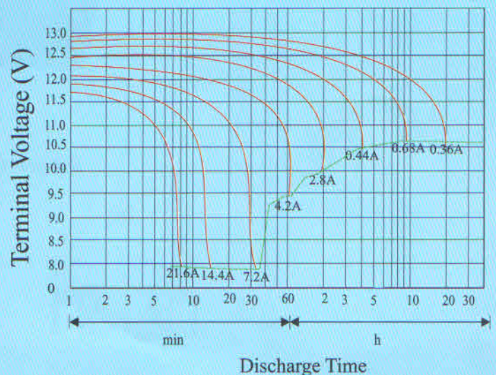
DISCHARGE CURRENT VS TIME 25! aC (77!a)
